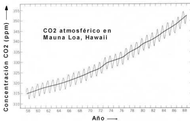
Fig. 3: Time series of the atmospheric \text{CO}_2 concentration as measured at Mauna Loa Observatory, Hawaii (From Peixoto and Oort, 1992). These data are accepted to be representative for the global trend. Fig. 4 shows that the continually rising \text{CO}_2 - trend does not fit the up - and down course of observed climate.
